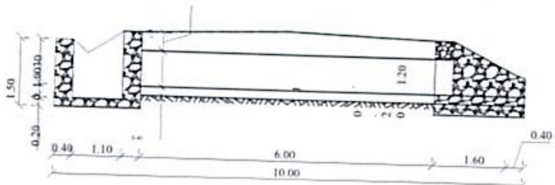
LONGITUDINAL CROSS-SECTION
